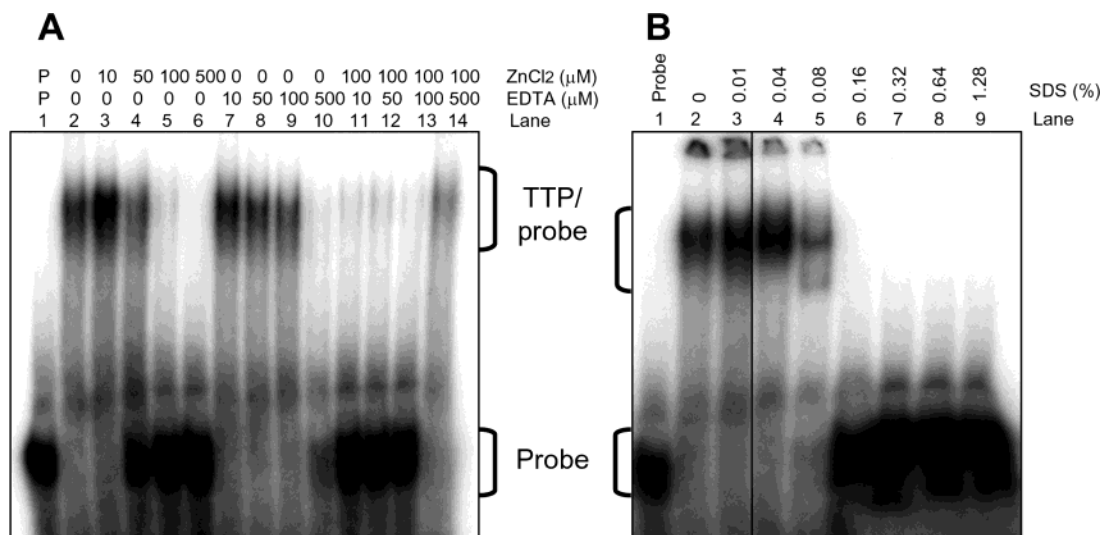
FIGURE 6: Effect of zinc, EDTA, and SDS on the ARE binding activity of TTP. ARE binding activity was assayed by GMSA using TTP (1 μL) purified by Ni-NTA beads and eluted with 100 mM imidazole buffer as described in the legend of Figure 4A (lane 6). The positions of TTP–probe complexes and free probes are indicated. (A) Effect of zinc and EDTA. GMSA buffers contained various concentrations of ZnCl 2 , EDTA, or mixtures of ZnCl 2 and EDTA as indicated. (B) Effect of SDS. GMSA buffers contained various concentrations of SDS as indicated.
