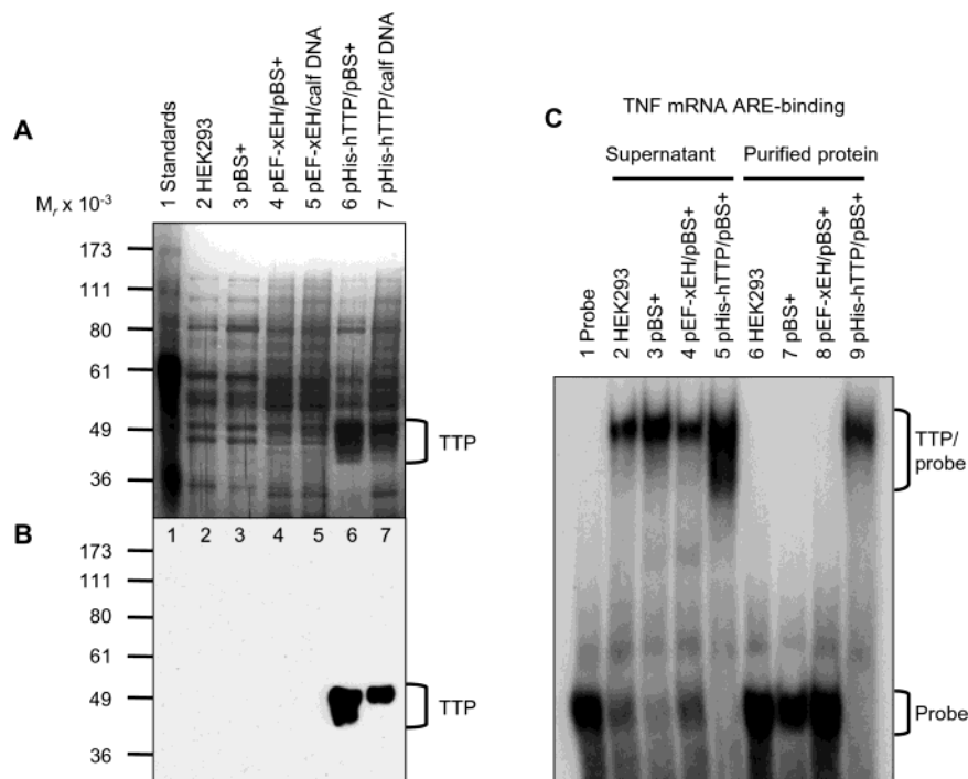
FIGURE 4: Identification of purified TTP free of endogenous ARE binding activity. HEK293 cells were transiently transfected with pHIS-hTTP (0.5 \mu g) and cotransfected with 4.5 \mu g of pBS+ (lane 6) or calf thymus DNA (lane 7). As negative controls, cells were also transfected with buffers only (lane 2), pBS+ only (5 \mu g) (lane 3), or pEF-xEH encoding a His-tagged Xenopus EH domain of intersectin (0.5 \mu g) and cotransfected with 4.5 \mu g of pBS+ (lane 4) or calf thymus DNA (lane 5). Proteins were purified with Ni-NTA beads. (A) Silver staining. Each lane was loaded with 5 \mu L of the purified proteins eluted with 100 mM imidazole buffer. (B) Immunoblotting. Each lane was loaded with 5 \mu L of the 10000g supernatant and detected with the anti-MBP-hTTP antibodies. (C) Gel mobility shift assay. Each assay used 4 \mu L of the 10000g supernatant (lanes 2–5) or 4 \mu L of the purified proteins in 100 mM imidazole elution buffer (lanes 6–9). The positions of TTP, TTP–probe complexes, and free probes are indicated.
