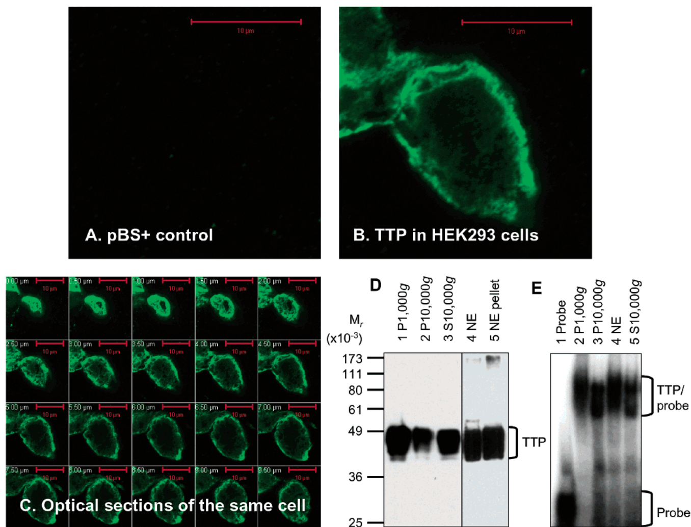
FIGURE 2: Expression and localization of active TTP in transfected human cells. (A–C) Expression and localization of TTP by immunocytochemistry. HEK293 cells were transfected with pBS+ control plasmid (A) and pHis-hTTP plasmid (B and C). The cells were immunostained with the anti-MBP-hTTP serum (1:5000 dilution) and labeled with goat anti-rabbit Alexa Fluor 488 (1:1000 dilution). Immunofluorescence was recorded with a confocal microscope as either a single image (A and B) or serial images of optical sections of a single cell with a 0.5 \mu m interval (C). (D) Expression and localization of TTP by immunoblotting. HEK293 cells were transfected with pHis-hTTP. The lysate was centrifuged at 1000g, resulting in S1000g and P1000g. S1000g was further centrifuged at 10000g, resulting in S10000g and P10000g. P1000g was extracted with a buffer containing 0.45 M KCl and centrifuged at 10000g, resulting in the 10000g supernatant (nucleic extract, NE) and the 10000g pellet (NE pellet). Proteins (8 \mu L) were separated by 10% SDS–PAGE, transferred onto a nitrocellulose membrane, and detected with the anti-MBP–hTTP serum. The position of TTP is indicated. The S10000g lane was loaded with proteins extracted from 10% of the cells used for other samples. (E) ARE binding activity by EMSA. The ARE binding activity was assayed by using proteins prepared as described for panel D. Each assay used 1 \mu L of each fraction. The positions of TTP–probe complexes and free probes are indicated.
