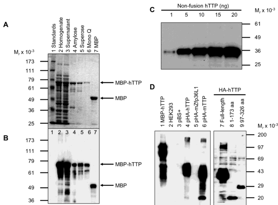
FIGURE 1: Purification of MBP-hTTP from E. coli and characterization of anti-MBP-hTTP antibodies. (A) Purification of MBP-hTTP stained with Coomassie blue: lane 1, protein size standards; lane 2, homogenate (50 \mu g of protein); lane 3, supernatant (50 \mu g); lane 4, amylose resin fraction (5 \mu g); lane 5, Superose 12 fraction (2 \mu g); lane 6, Mono Q fraction (1 \mu g); and lane 7, MBP eluted from the amylose resin column (5 \mu g). The positions of MBP-hTTP and MBP are indicated. (B) Detection of MBP-hTTP with anti-MBP serum. The samples were identical to those in panel A except that \sim 10% of the amount of protein was used in each lane. (C) Detection limit of anti-MBP-hTTP serum by Western blotting. Nonfusion hTTP purified from E. coli as shown in Figure 7A (lane 2) (1, 5, 10, 15, and 20 ng) as indicated was probed with the anti-MBP-hTTP serum (1:10000) for 1 h and with GAR-HRP (1:10000) for 30 min and exposed to X-ray film for 1 min. (D) Characterization of the anti-MBP-hTTP serum by Western blotting. Protein samples were probed with the anti-MBP-hTTP serum (1:10000) for 1 h and with GAR-HRP (1:10000) for 1 h and exposed to X-ray film for 1 min: lane 1, purified MBP-hTTP (50 ng); lane 2, untransfected HEK293 cell extract (50 \mu g); lane 3, pBS+ transfection extract (50 \mu g); lane 4, pHA-hTTP transfection extract (50 \mu g); lane 5, pHA-mZfp36L1/mTIS11b transfection extract (50 \mu g); lane 6, pHA-mTTP transfection extract (50 \mu g); lane 7, transfection extract with full-length hTTP (50 \mu g); lane 8, transfection extract with amino-terminal residues 1–173 of hTTP (50 \mu g); and lane 9, transfection extract with carboxyl-terminal residues 97–326 of hTTP (50 \mu g).
