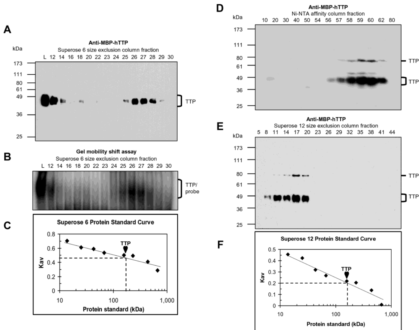
FIGURE 5: Size of active TTP from transfected human cells. The size of TTP was estimated by size exclusion chromatography using the Superose 6 column and the 10000g supernatant from HEK293 cells transfected with pHIS-hTTP (A–C) and using the Superose 12 column and TTP purified by a Ni-NTA affinity column from HEK293T cells transfected with pHIS-hTTP (D–F). Fractions were analyzed for the presence of TTP by immunoblotting with anti-MBP-hTTP antibodies (A, D, and E) and analyzed for ARE binding activity by GMSA (B). Lane L in panels A and B represents the initial proteins loaded in the size exclusion columns. The positions of TTP and TTP–probe complexes are indicated. The size of TTP was estimated using a standard curve generated with protein standards run on the same column under identical conditions (C and F), in which K_{av} = (V_e - V_o)/(V_t - V_o) , where V_e , V_o , and V_t are the elution volume of the protein determined by the experiment, the void volume determined with blue dextran (2000 kDa), and the bed volume of the column provided by the manufacturer (Amersham), respectively. The protein standards that were used were provided by the manufacturer (Amersham): bovine pancreas ribonuclease A (13.7 kDa), bovine pancreas chymotrypsinogen (25 kDa), hen egg ovalbumin (43 kDa), bovine serum albumin (67 kDa), rabbit muscle aldolase (158 kDa), bovine liver catalase (232 kDa), horse spleen ferritin (440 kDa), and bovine thyroid thyroglobulin (669 kDa). Similar results were obtained using the Superose 12 column and the same extracts as in panels A–C (data not shown).
