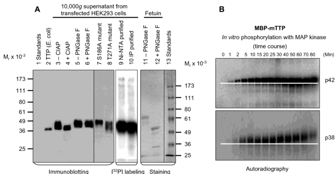
FIGURE 8: Phosphorylation of TTP in vivo and in vitro . (A) The 10000g supernatant from HEK293 cells transfected with wild-type pHIS-hTTP was treated with or without CIAP (lanes 3 and 4) or with or without PNGase F (lanes 5 and 6). Nonfusion hTTP purified from E. coli cells as shown in Figure 7A (lane 2) was used as a size standard for estimating the extent of the dephosphorylation (lane 2). HEK293 cells transfected with the wild-type plasmid were also labeled with [ 32 P]orthophosphate in vivo . TTP was then purified from the 10000g supernatant of the labeled cells by affinity purification using Ni-NTA beads (lane 9) or by immunoprecipitation using the anti-MBP-hTTP serum (lane 10). The 10000g supernatants from HEK293 cells transfected with two mutant plasmids (S186A and T271A) are also shown (lanes 7 and 8). Proteins were separated by 10% SDS-PAGE, and TTP was detected with anti-MBP-hTTP antibodies (lanes 2–8). The labeled protein was detected by autoradiography (lanes 9 and 10). As a positive control for deglycosylation, fetuin was treated with or without PNGase F under identical conditions and detected with Coomassie blue staining (lanes 11 and 12). (B) Phosphorylation of MBP-mTTP by MAP kinases in vitro . MBP-mTTP (1 \mu M) purified from E. coli by amylose affinity resin was treated with MAP kinases, including p42/ERK2 (top) and p38 (bottom). Aliquots of the reaction mixtures were taken at various times as indicated and separated by 10% SDS-PAGE. The gels were exposed to X-ray film. A white line on the image highlights the gel mobility shift of the phosphorylated protein. Similar results were obtained with JNK, and with MBP-hTTP as the substrate (data not shown).
